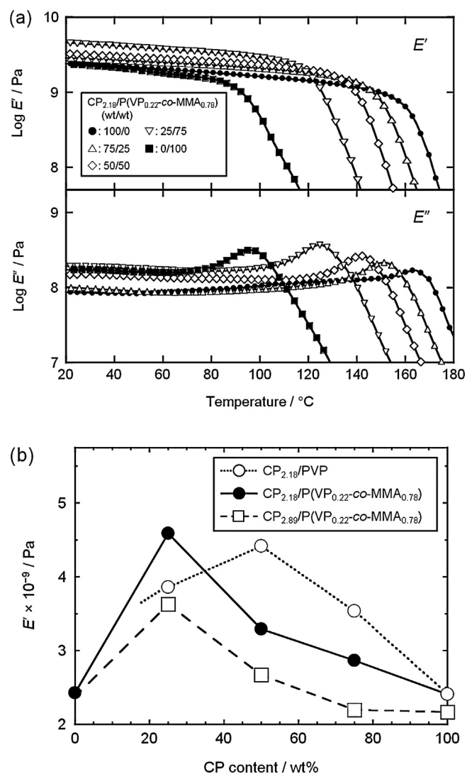
Fig. 7. (a) Temperature dependence of the dynamic storage modulus E' and loss modulus E'' for \text{CP}_{2.18}/\text{P}(\text{VP}_{0.22}\text{-co-MMA}_{0.78}) blends, and (b) the glassy state E' value (measured at 20^\circ\text{C} ) vs. composition plots for three series of blends, \text{CP}_{2.18}/\text{PVP} , \text{CP}_{2.18}/\text{P}(\text{VP}_{0.22}\text{-co-MMA}_{0.78}) , and \text{CP}_{2.89}/\text{P}(\text{VP}_{0.22}\text{-co-MMA}_{0.78}) .
