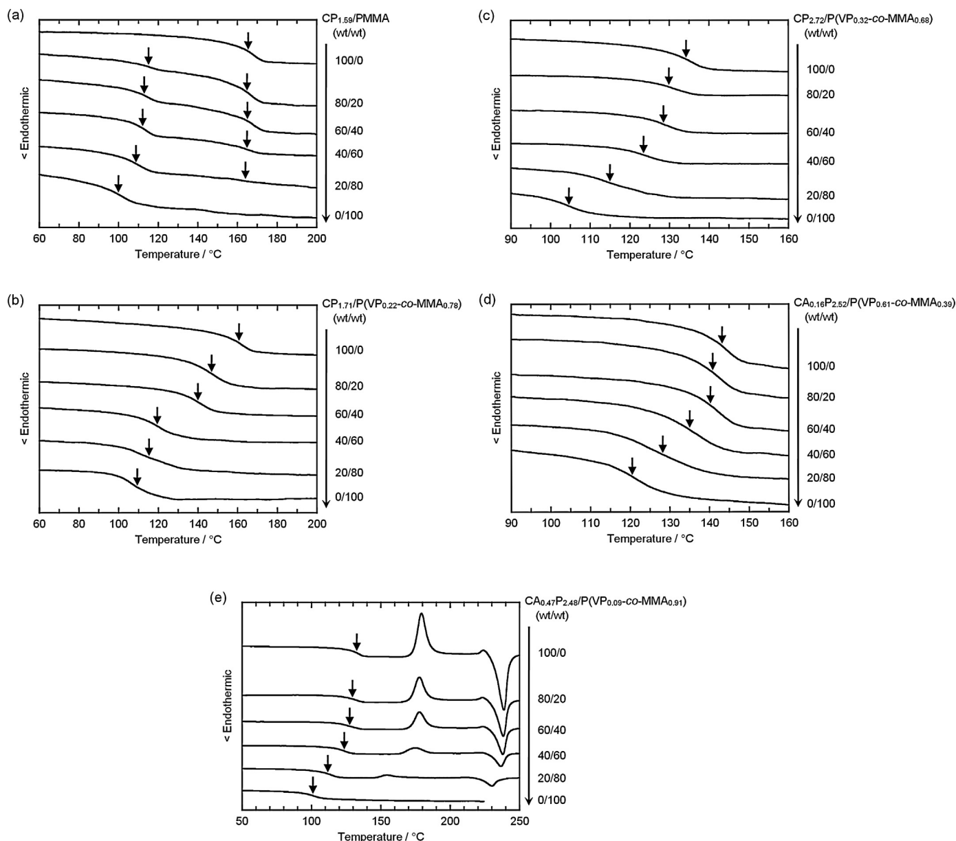
Fig. 3. DSC thermograms obtained for (a) CP 1.59 /PMMA, (b) CP 1.71 /P(VP 0.22 -co-MMA 0.78 ), (c) CP 2.72 /P(VP 0.32 -co-MMA 0.68 ), (d) CA 0.16 P 2.52 /P(VP 0.61 -co-MMA 0.39 ), and (e) CA 0.47 P 2.48 /P(VP 0.09 -co-MMA 0.91 ) blends. Arrows indicate a T_g position taken as the midpoint of a baseline shift in heat flow.
