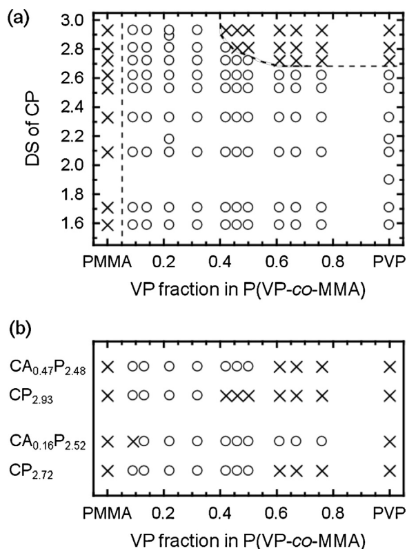
Fig. 2. (a) Miscibility map for the blend system CP/P(VP-co-MMA), depicted as a function of DS of CP and VP fraction in P(VP-co-MMA), and (b) miscibility estimation for CAP/P(VP-co-MMA) blends using partially acetylated CA 0.16 P 2.52 and CA 0.47 P 2.48 as a function of VP fraction in P(VP-co-MMA), in comparison with the corresponding CP/P(VP-co-MMA) blends using CP 2.72 and CP 2.93 , respectively. Symbols indicate that a given pair of CP or CAP/P(VP-co-MMA) is miscible (O) or immiscible (X).
