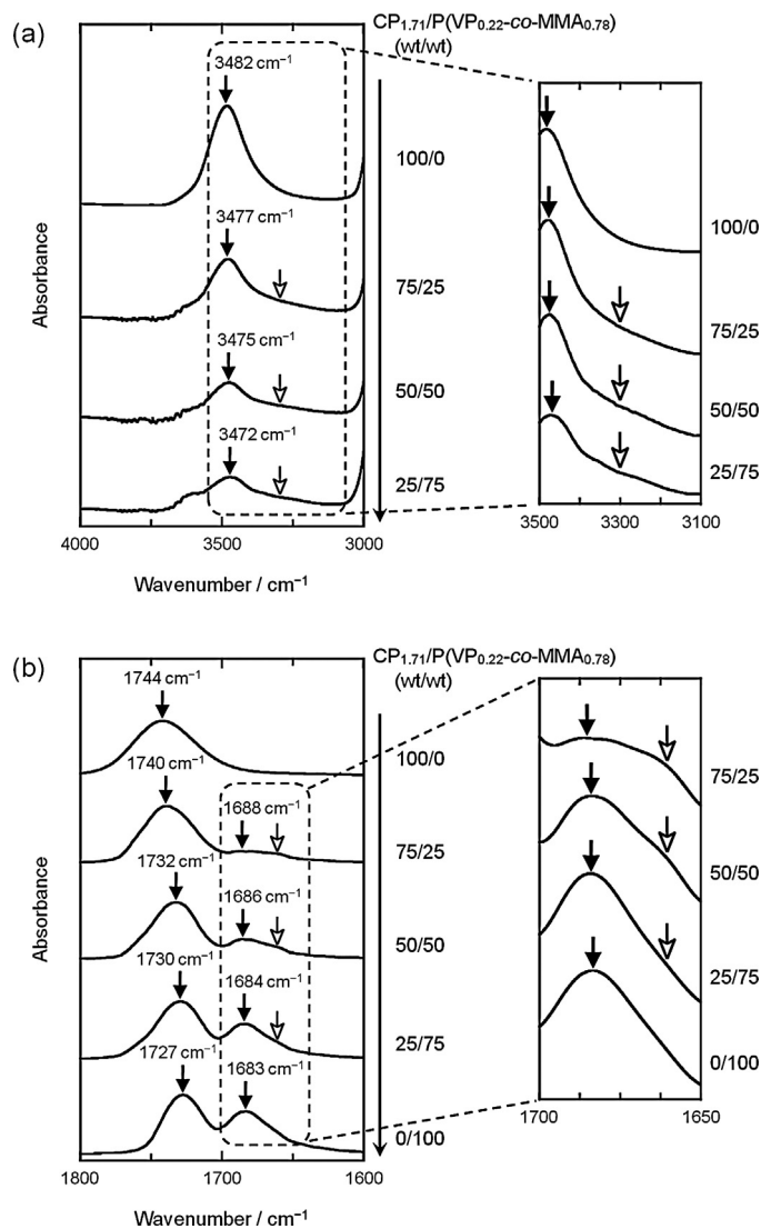
Fig. 4. FT-IR spectra of CP 1.71 , P(VP 0.22 -co-MMA 0.78 ), and their blends in the frequency regions of (a) O–H and (b) C=O stretching vibrations. Data in the ranges of 3100–3500 cm -1 and 1650–1700 cm -1 are also shown on an enlarged scale. Solid arrows indicate a peak-top position in the respective specific absorption bands, and white arrows indicate a shoulder band associated with hydrogen bonding (see text for discussion).
