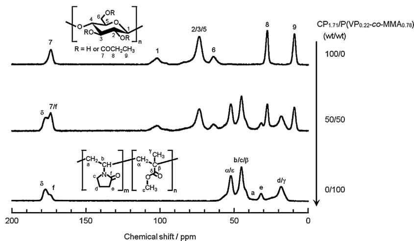
Fig. 5. Solid-state ^{13}\text{C} CP/MAS NMR spectra for CP 1.71 , P(VP 0.22 -co-MMA 0.78 ), and their 50/50 blend.
