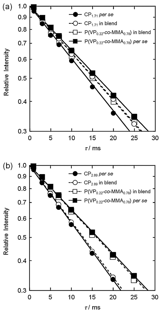
Fig. 6. Semilogarithmic plots of the decay of ^{13}\text{C} resonance intensities as a function of spin-locking time \tau , for solid films of (a) \text{CP}_{1.71} , \text{P}(\text{VP}_{0.22}\text{-co-MMA}_{0.78}) , and their 50/50 blend, and (b) \text{CP}_{2.89} , \text{P}(\text{VP}_{0.22}\text{-co-MMA}_{0.78}) , and their 50/50 blend. The monitoring was conducted for the peak intensity of C2/C3/C5 pyranose carbons of CP and that of \text{C}_b/\text{C}_c/\text{C}_\beta carbons of the copolymer (see Fig. 5).
