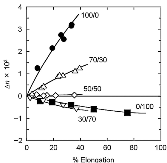
Fig. 8. Plots of birefringence \Delta n vs. % elongation for drawn films of CP 2.09 /P(VP 0.46 -co-MMA 0.54 ) blends.
